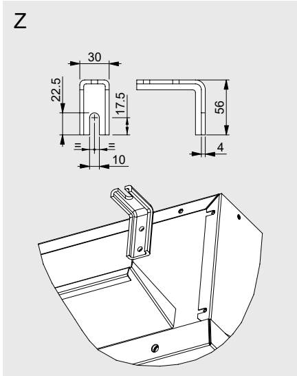
Positioning of electric heaters
