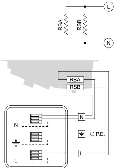
Standardmodell
