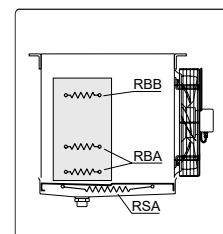
Positioning of electric heaters
