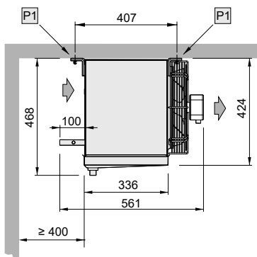
Fastening detail
