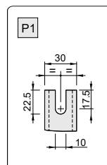
Fastening detail
