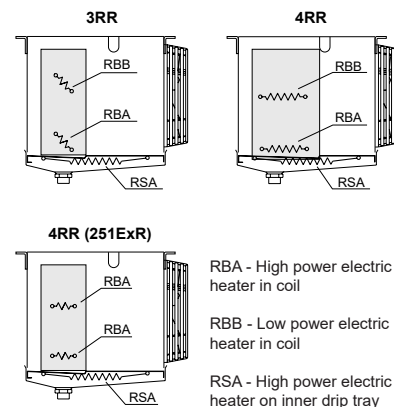
Positioning of electric heaters
