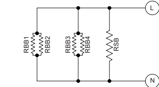
230V/1/50-60Hz connection to be set
