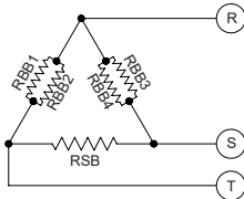
230V/3/50-60Hz connection to be set
