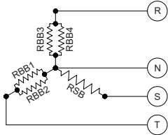
400V/3/50-60Hz connection STANDARD
