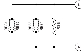
230V/1/50-60Hz connection to be set
