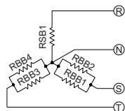
400V/3/50-60Hz connection STANDARD
